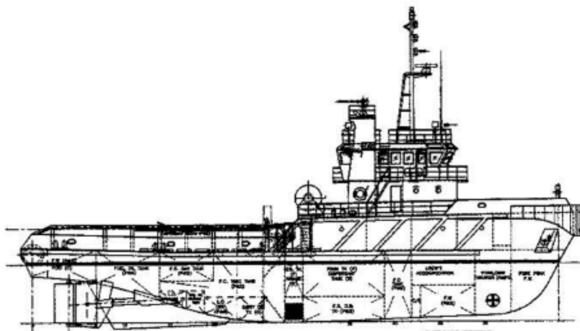
OUTBOARD PROFILE
