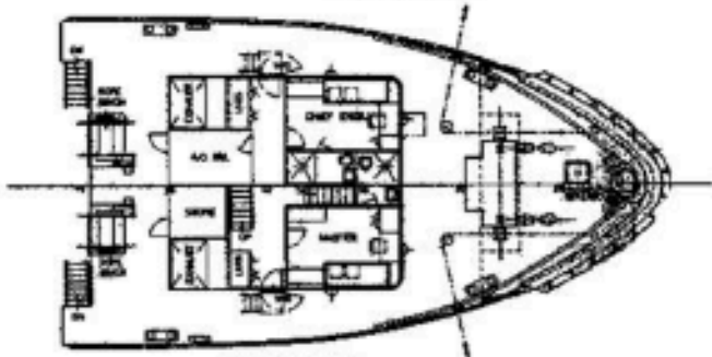
FORECASTLE DECK
